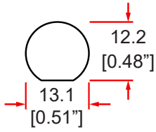
BNC Hole Patterns
