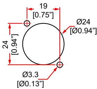
D-Series Hole Patterns
